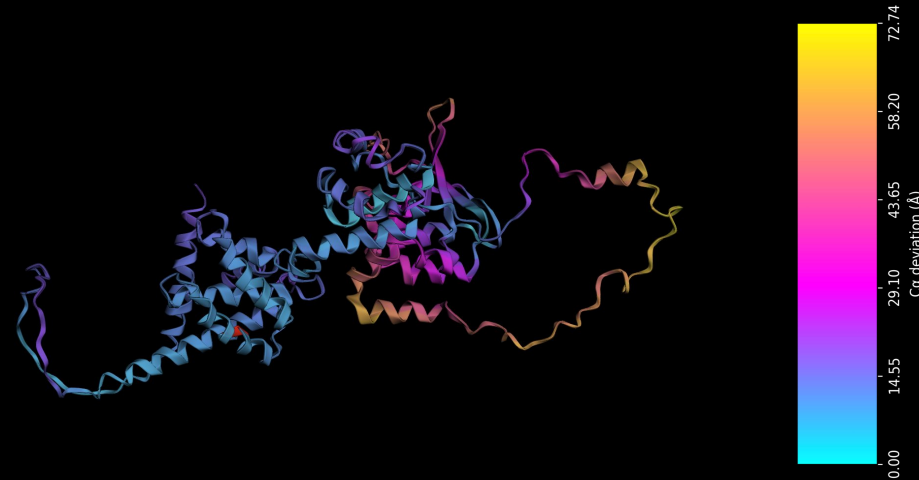
9. DnaB Original structure coloured by deviations from Mutant
