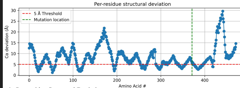
6. Per-residue Structural Deviation
