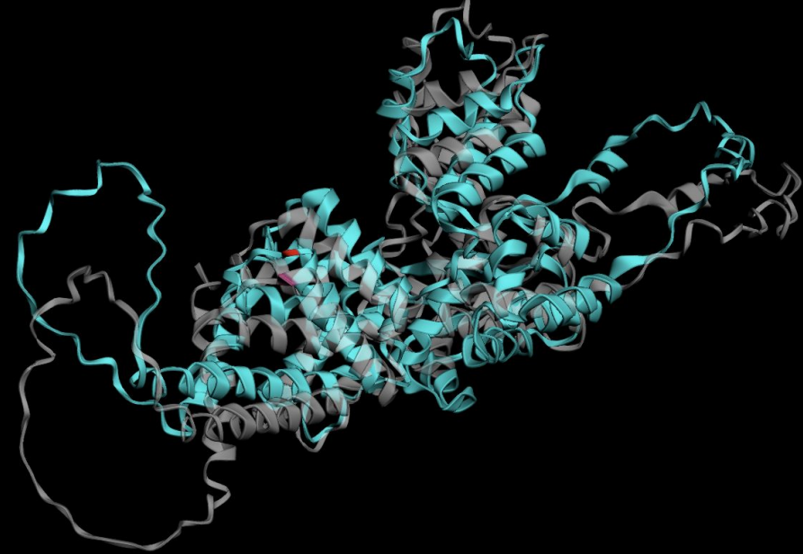
5. DnaB Original structure superimposed on Mutant
