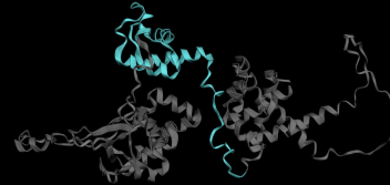
3. DDBH2-1
