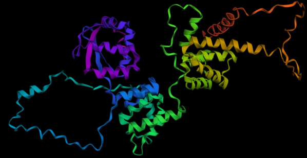
1. ColabFold Structure of DnaB
